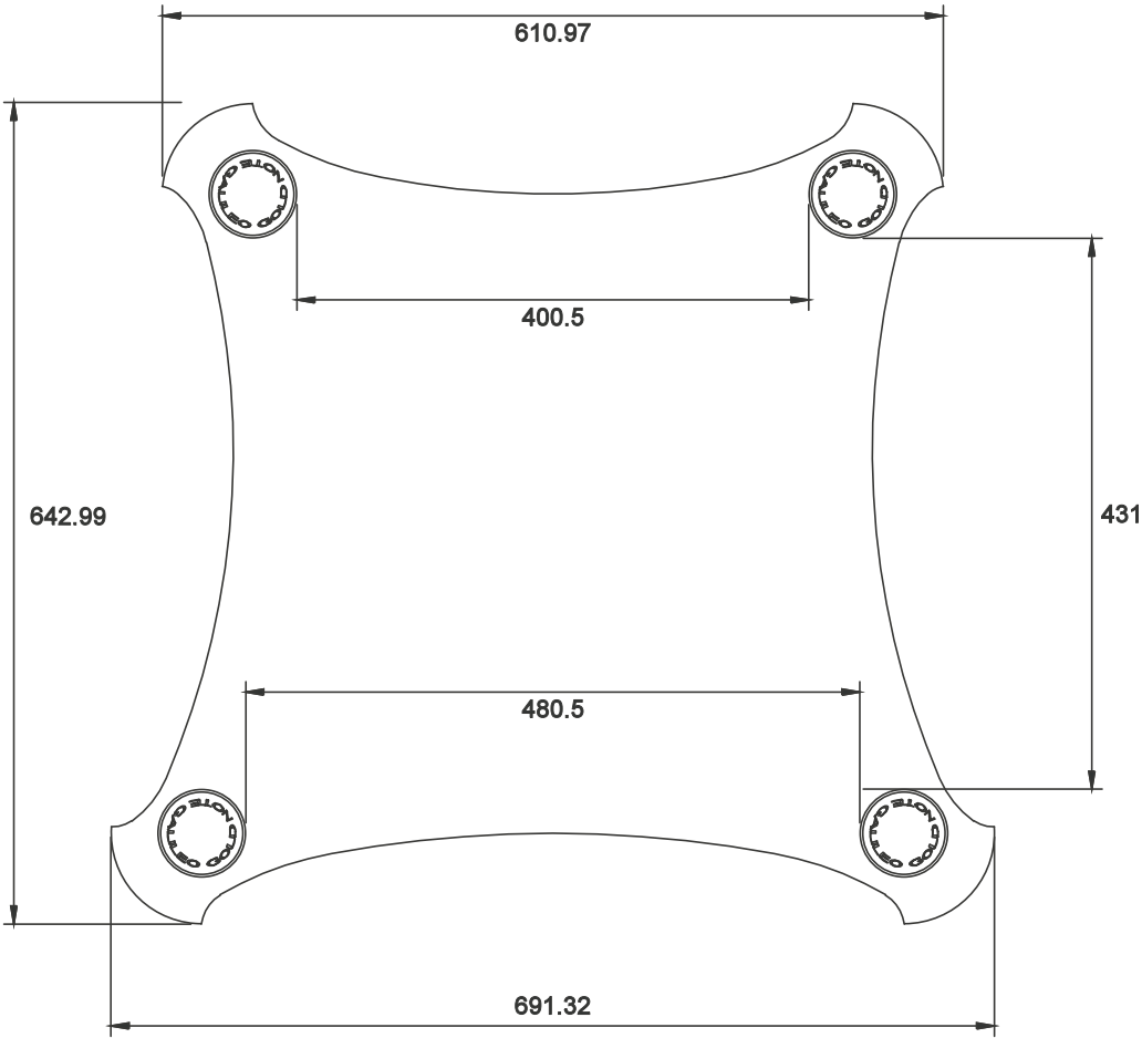
TOP PANEL VIEW
