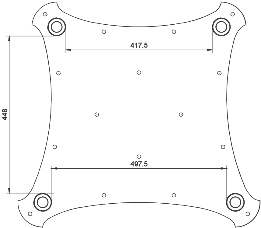
BOTTOM PANEL VIEW
